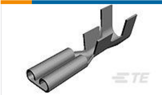
TE 产品编号61368-1 FASTON .250 REC 24-20 AWG TPBR
