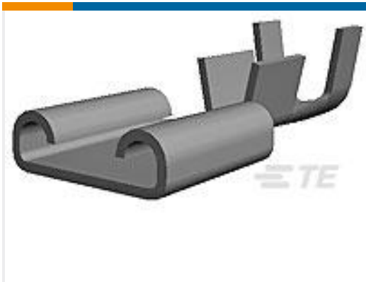
TE 产品编号170183-1 250 FASTON,REC.,22-18 AWG,BR
