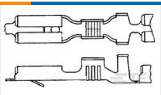
TE 产品编号170015-2 FF 110 REC 20-16AWG BR REREELING
