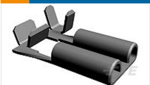
TE 产品编号1742049-1 187 FASTON,FLAG,REC.,(2X)18 AWG, NPST
