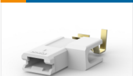
TE 产品编号1969109-1 ULTRA-POD 250 ASSY REC 18-14 AWG BR
