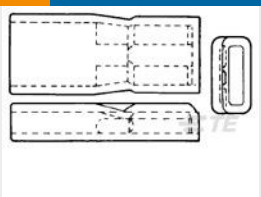
TE 产品编号174817-2 250 sleeve PL YELLOW transparent
