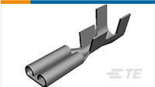
TE 产品编号170213-1 250 FASTON,REC.,18-14 AWG,BR
