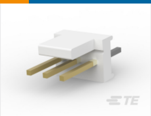
TE 产品编号1-640454-6 Polyester Vertical PCB Header: 2.54 mm, With Mating Alignment, Unshrouded
