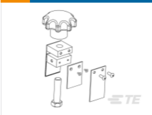
TE 产品编号1901850-1 ASSY, EXT TOOL, 25.4mm
