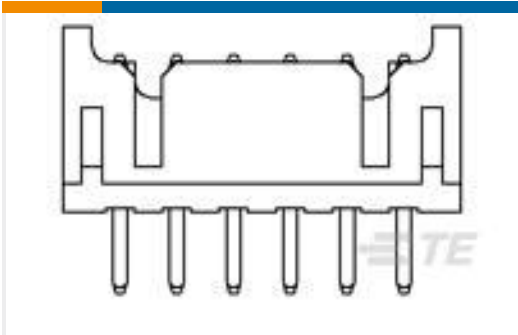
TE 产品编号1470109-8 2.0mm Pitch Header, Dip 8p
