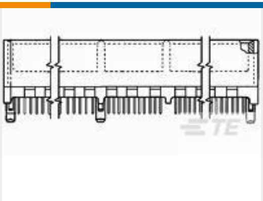
TE 产品编号1-5145166-2 STANDARD EDGE .050 SERIES 92 DUAL ASSY
