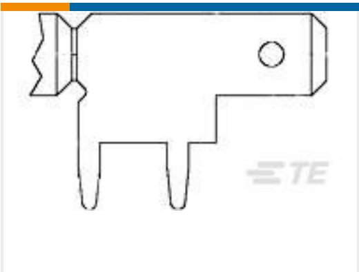
TE 产品编号1217061-1 187 FASTON,FLAG,TAB,TNBR
