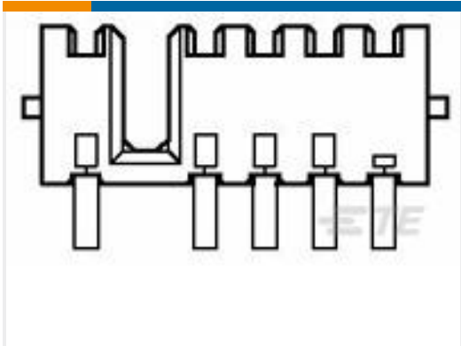
TE 产品编号1747367-1 RECEPTACLE ASSEMBLY 2.5MM PITCH BATTERY
