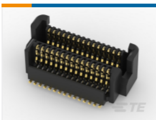
TE 产品编号2291283-1 0.5MM FPH BTB, 4H/30POS/15U/TR /WB/B
