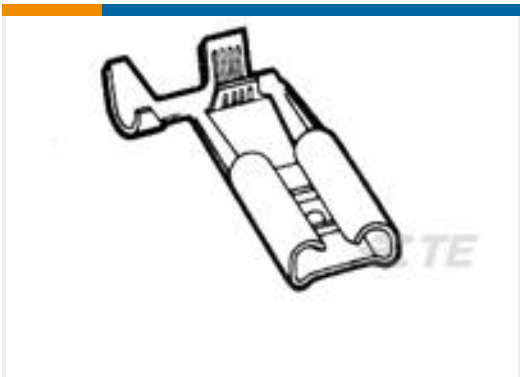
TE 产品编号180388-2 250 FASTON, REC., 20-16 AWG, TPBR
