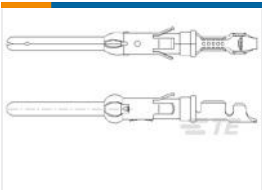
TE 产品编号1-163081-1 .062 DIA PIN ASSY 3+
