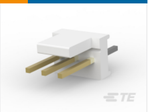
TE 产品编号1-640454-4 Polyester Vertical PCB Header: 2.54 mm, With Mating Alignment, Unshrouded
