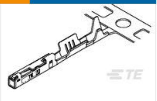
TE 产品编号1827855-3 0.50 SERIES CONNECTER RECEPTACLE CONTACT
