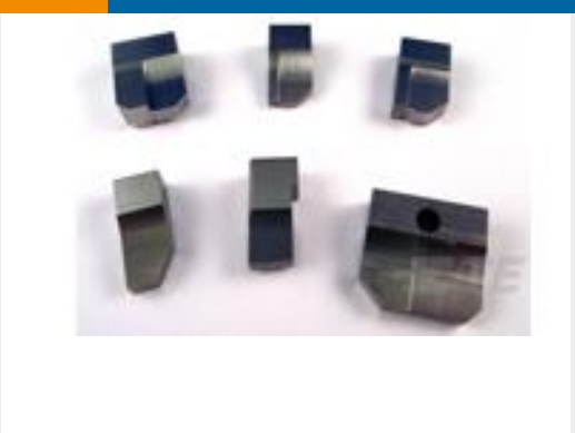
TE 产品编号1333205-6 ANVIL, COMBINATION (.090)
