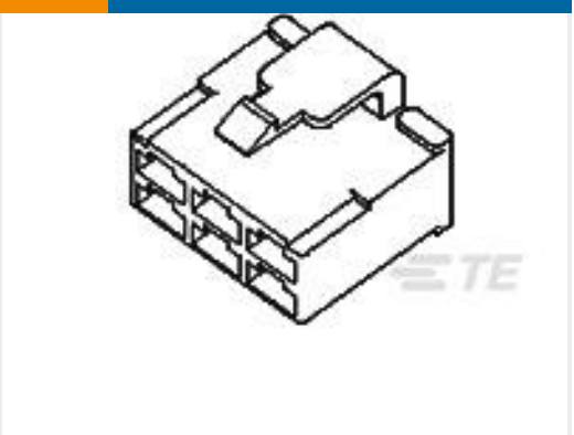
TE 产品编号172134-6 FF 250 PLUG HSG 4P NYLON GRAY
