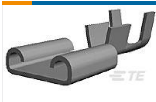
TE 产品编号1-160301-9 250 FASTON, REC., 10-12 AWG, PHBZ
