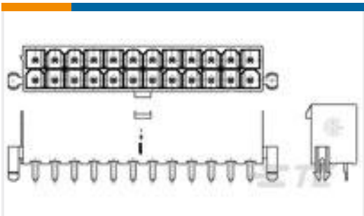
TE 产品编号1-1586039-6 16P VAL-U-LOK VRT HDR W/P V2
