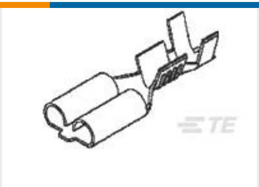
TE 产品编号170342-1 250 FASTON, REC., 20-14 AWG, BR
