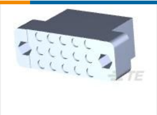
TE 产品编号205607-2 PIN BLK,15 POSN,AUTOWIRE
