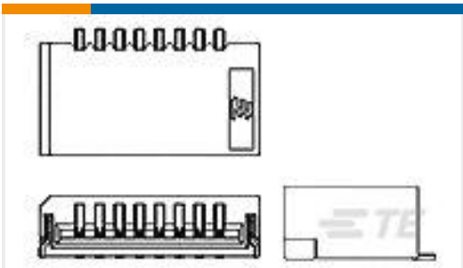
TE 产品编号1-84981-1 1MM FFC SMT H ASSY 11P EMBOSS
