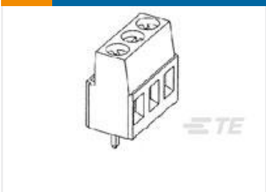
TE 产品编号1-282841-1 TERMI-BLOK PCB MOUNT 11P.5
