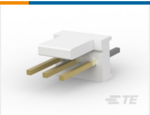
TE 产品编号1-640454-9 Polyester Vertical PCB Header: 2.54 mm, With Mating Alignment, Unshrouded
