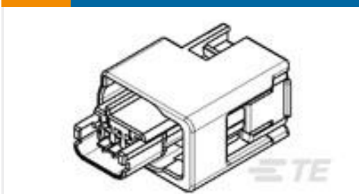
TE 产品编号1438454-1 0.64MM,3 POSN SEALED PLUG ASSY
