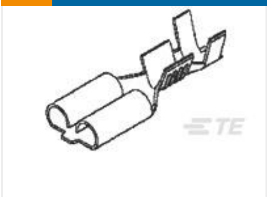
TE 产品编号170032-5 250 FASTON,REC.,20-14 AWG,TPBR
