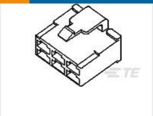
TE 产品编号172134-2 FF 250 PLUG HSG 4P NYLON BLACK
