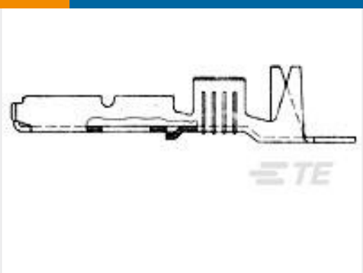
TE 产品编号281938-1 MIC MARKII RCPT CONTACT
