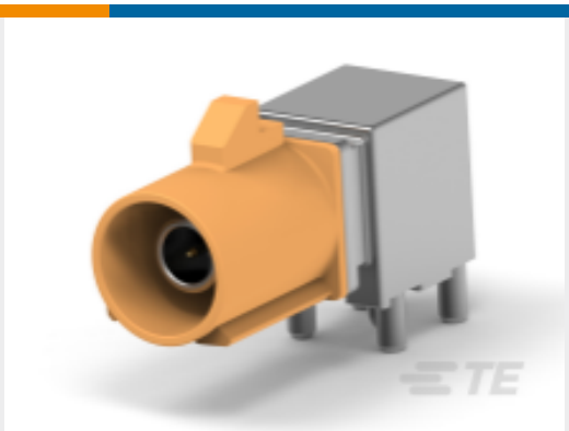
TE 产品编号1-2291392-2 MALE ASM, 1 POS, R/A, PCB, FAKRA
