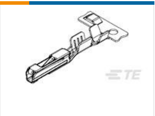
TE 产品编号1326028-4 0.64MM FEMALE CONTACT,AU, 22AWG
