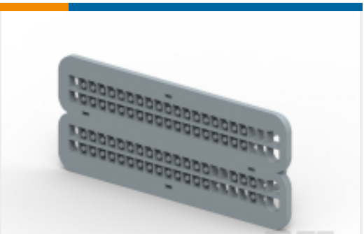
TE 产品编号5-284871-2 MULTIPLE CAVITY MASK FOR 94 POS. CONN.
