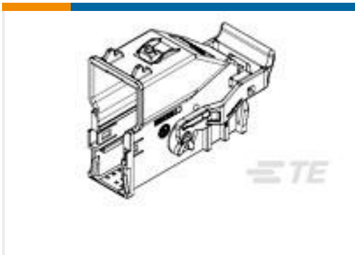
TE 产品编号1-1924337-3 Shield Assy, 54 POSN, 0.64mm, 20 DEG BLK
