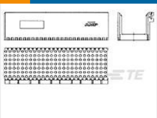
TE 产品编号352674-2 ZP,HSN 22MM LIF SHR
