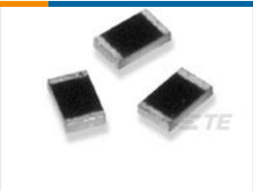
TE 产品编号2-1879280-6 RP 2A 169K 0.1% 15PPM 1K RL
