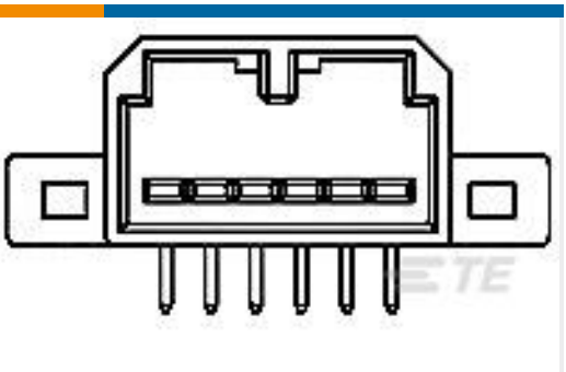
TE 产品编号175506-2 040 MLC CAP ASSY 6P
