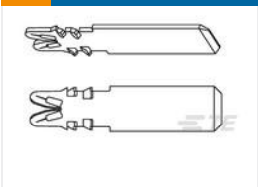
TE 产品编号1601072-5 .187 X .020 MULTI-BARB TAB SIA
