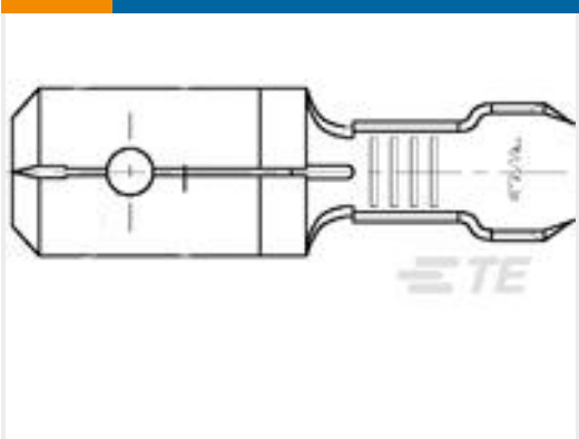
TE 产品编号626377-2 TERMINAL FASTON .250 TAB 22-18 AWG TPBR
