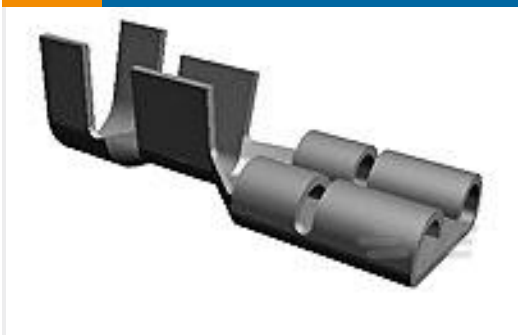
TE 产品编号1217917-2 250 FASTON,LIF REC.,18-14 AWG,BR
