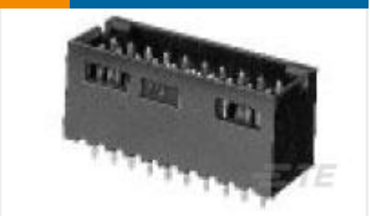
TE 产品编号1-103168-2 28 MODII HDR DRST SHRD .100CL
