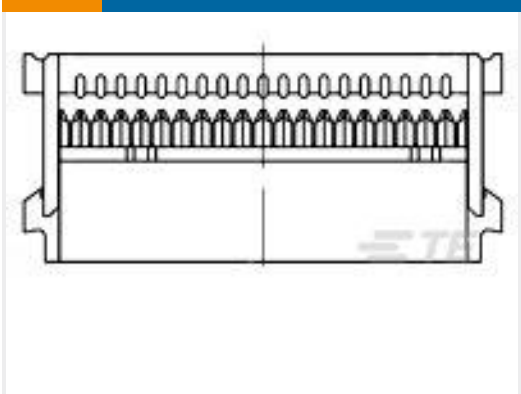
TE 产品编号1-1658526-5 609-2630LF FEM SOCKET, LEAD FREE
