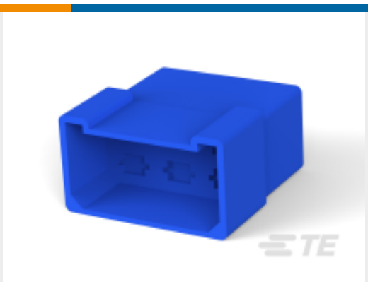
TE 产品编号1-171433-6 FF TAB HSG 6P NYLON BLUE
