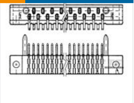
TE 产品编号3-582152-5 41 AMP BLADE HDR ASSY
