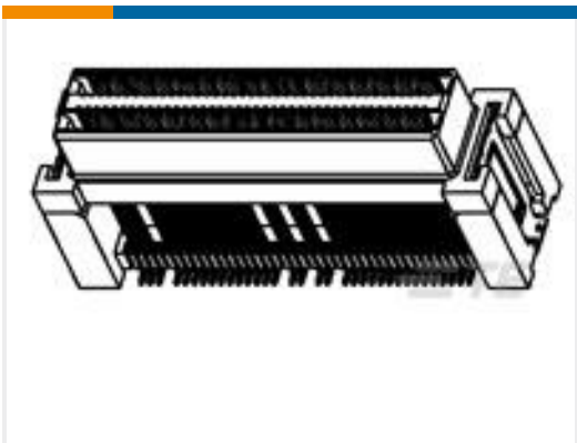
TE 产品编号6376608-2 MICRO STACK REC ASSY 80P WITH TAPE
