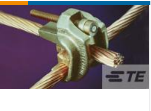
TE 产品编号83751-2 WRENCH-LOK 300-300, 500-3/0
