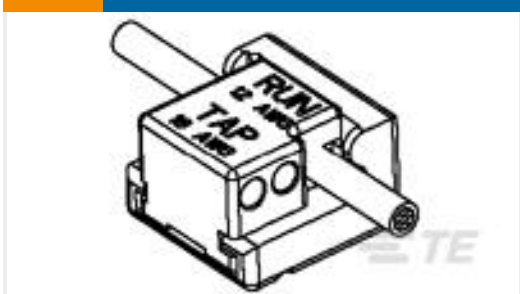
TE 产品编号1811027-1 ASSEMBLY,12AWG TAP
