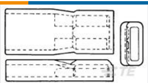
TE 产品编号174817-1 POSITIVE LOCK 250 (6.3 MM) SLEEVE
