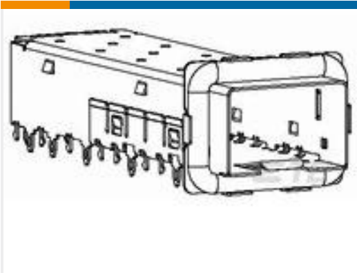
TE 产品编号2057086-2 SFP+ Enhanced 1x1 Cage Assembly
