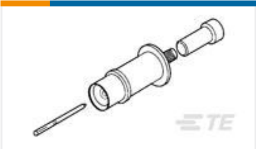
TE 产品编号225792-5 ARINC SIZE 3 SOCKET
