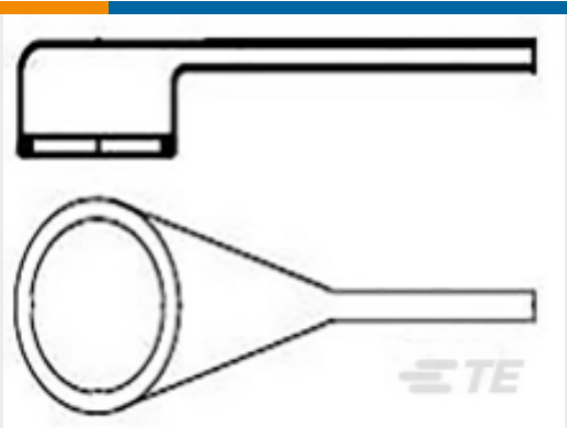
TE 产品编号813350-000 Heat Shrink Boots: Lipped, Right Angle
