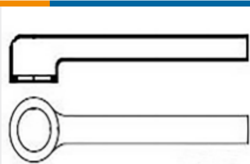
TE 产品编号269741-000 Low Profile Heat Shrink Boots: Blow Mold, Lipped, Right Angle
