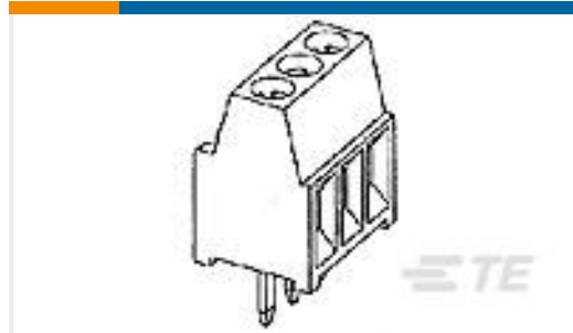
TE 产品编号1546215-7 TERMI-BLOK PCB MOUNT, 90 7P.
